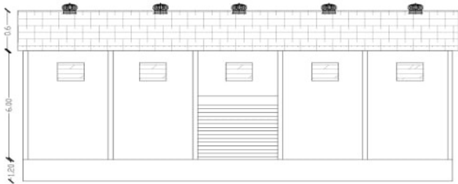
ELEVATION SCALE 1:100
