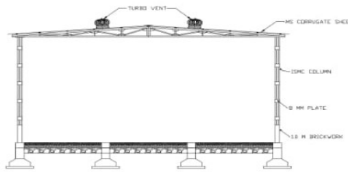
SECTION X-X' SCALE 1:100
